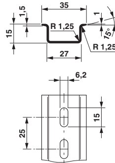
Dimensional drawing
