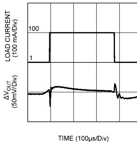
Load Transient
