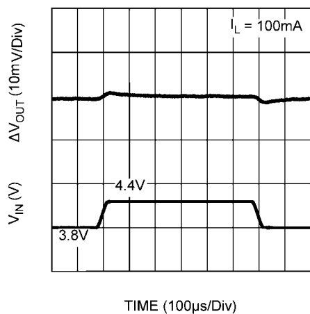
Line Transient
