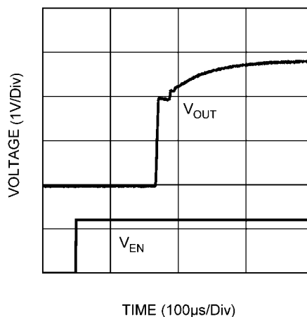
Enable Start-up Time, ( I_L = 1mA , V_{OUT} = 2.8V )
