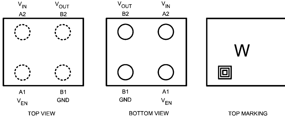
4-Bump Thin micro SMD Package and Extreme Thin micro SMD Package, Large Bump NS Package Number TLA04/XRA04
