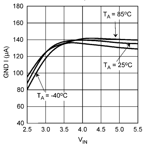
Ground Current vs V_{IN} , I_{LOAD} = 100mA
