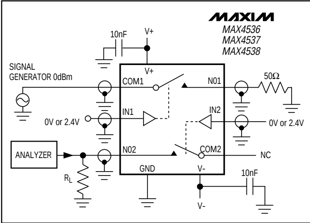
Figure 5. Crosstalk
