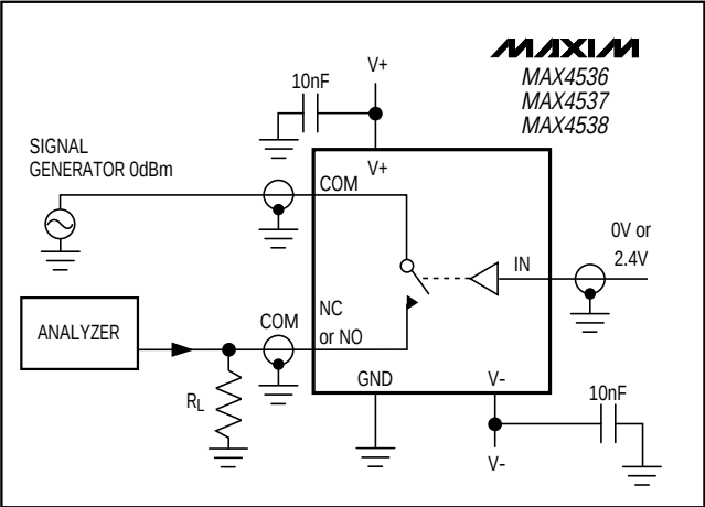
Figure 4. Off Isolation
