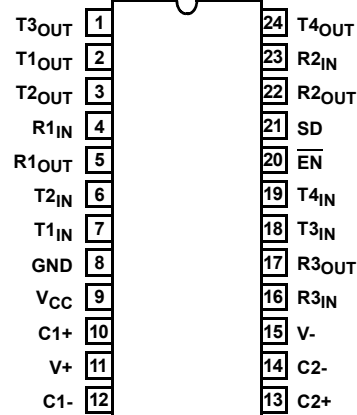
HIN206 (SOIC) TOP VIEW
