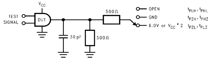
FIGURE 1. AC Test Circuit
