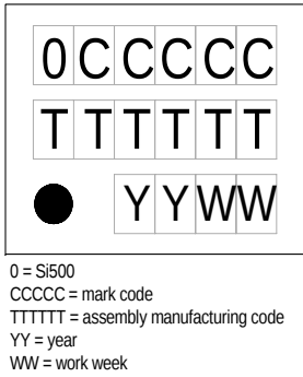
Figure 2. Top Mark
