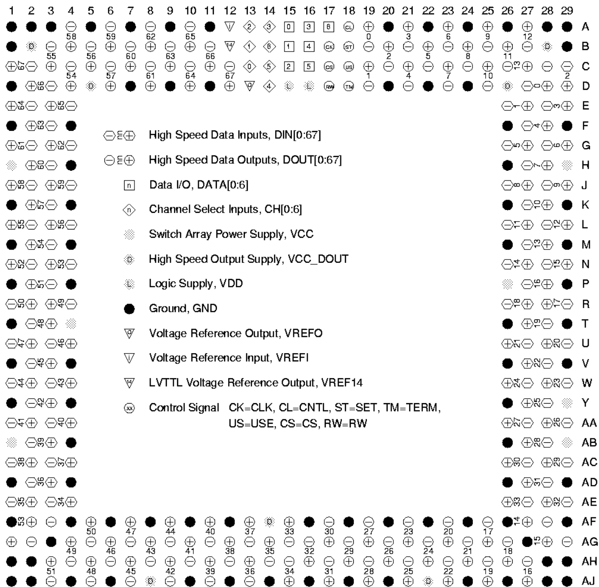
Figure 9. HDMP-3268 pin locations.
