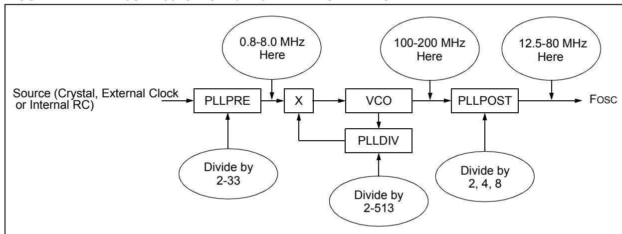
FIGURE 7-2: dsPIC33FJ12GP201/202 PLL BLOCK DIAGRAM
