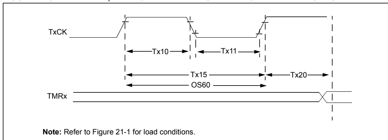
FIGURE 21-5: TIMER1, 2 AND 3 EXTERNAL CLOCK TIMING CHARACTERISTICS
