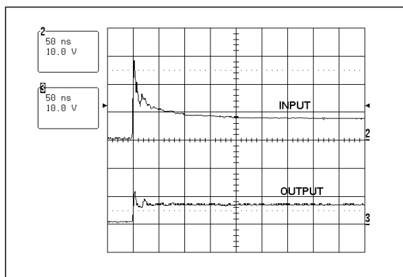
Fig. A5: Remaining voltage at the input and output of the device during a \pm 16\text{kV} ESD surge (IEC61000-4-2).
