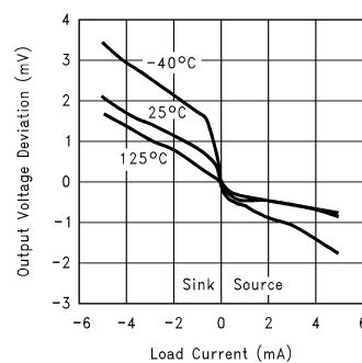
Load Regulation
