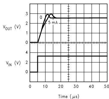
Start-Up Response
