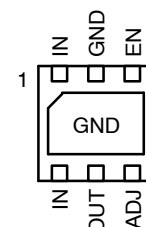
NCP691, NCP692 – DFN6 Adjustable Version (Bottom View)
