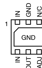
NCP690, NCV8690 – DFN6 Adjustable Version (Bottom View)
