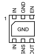
NCP691, NCP692 – DFN6 Fixed Version (Bottom View)
