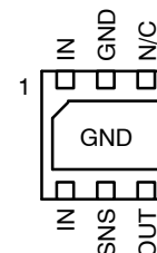
NCP690, NCV8690 – DFN6 Fixed Version (Bottom View)
