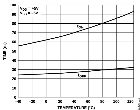
Figure 12. t_{ON}/t_{OFF} Times vs. Temperature, Dual Supplies
