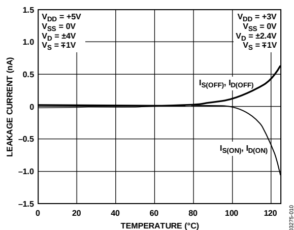
Figure 10. Leakage Current vs. Temperature, Single Supply
