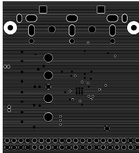
Figure 19: EVAL-ADV7390/91EBZ Ground Plane Layer 2
