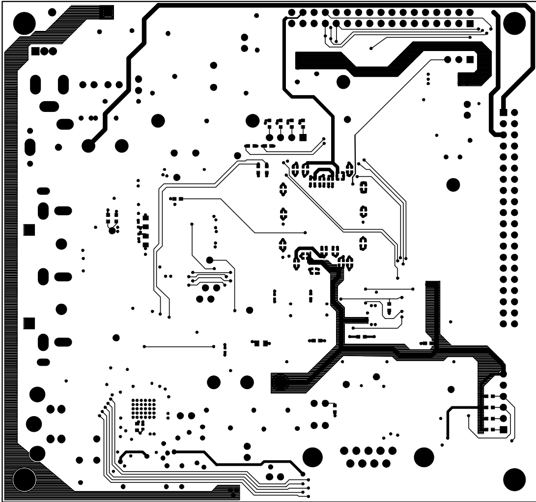
Figure 9: EVAL-ADV739xFEZ Layer 4
