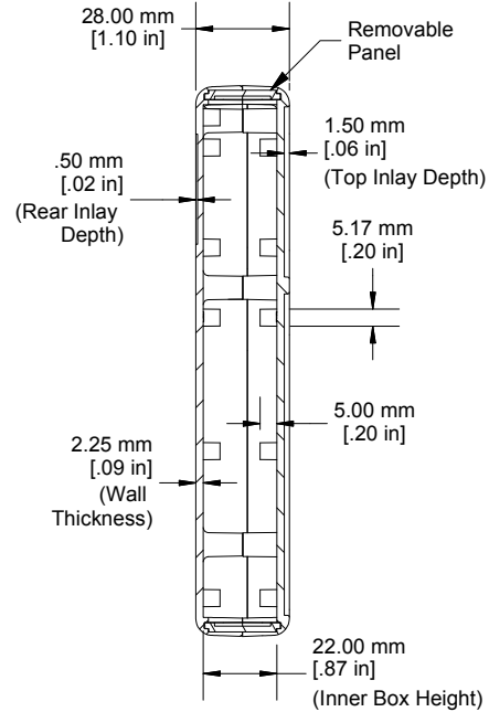
SECTION A-A (Side View of Assembly)
