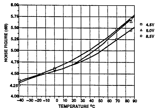
Figure 11. Noise Figure
