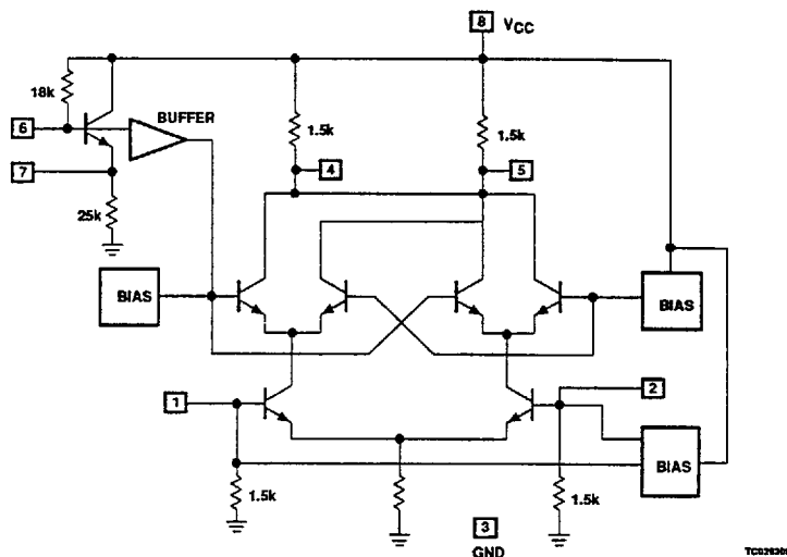
Figure 2. Equivalent Circuit
