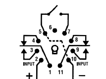
48K91US (dotted line represents internal connection)
