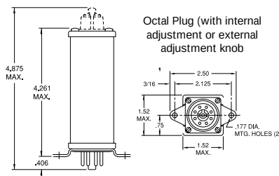
Chassis Mount —4, —5
