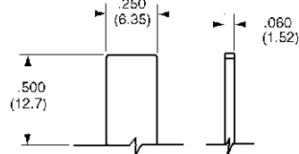
Terminal Detail
