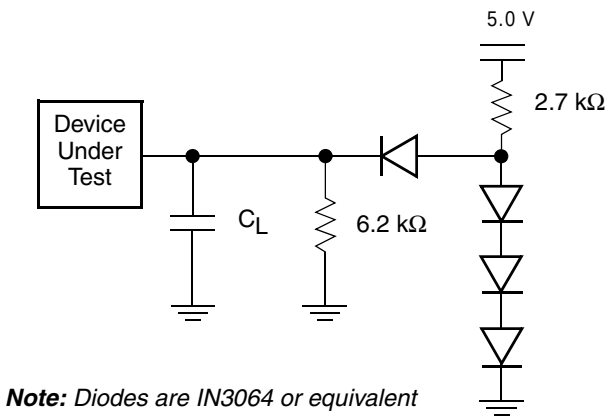
Figure 7. Test Setup
