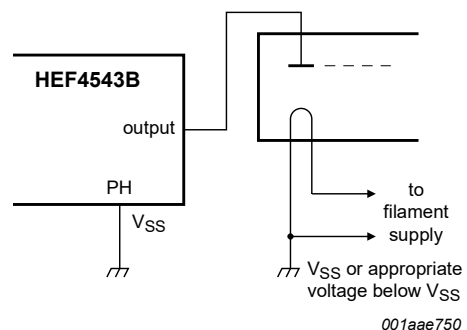
Fig. 11. Connection to fluorescent display readout
