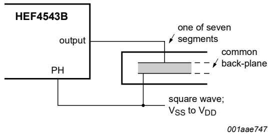
Fig. 8. Connection to LCD readout
