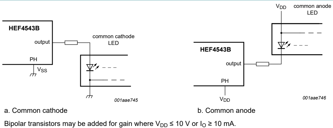
Fig. 7. Connection to LED display readout
