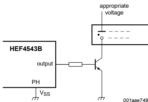
Fig. 10. Connection to gas discharge display readout
