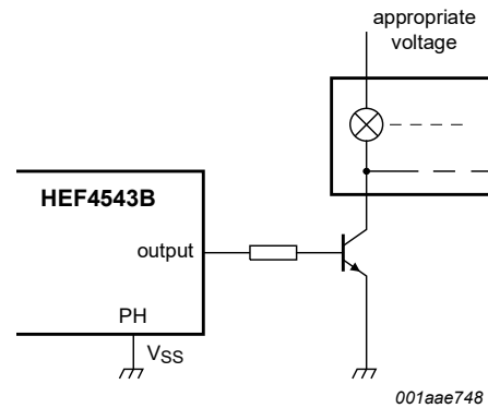
Fig. 9. Connection to incandescent display readout
