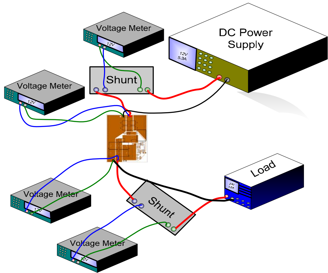
Figure 6: Test Procedure Set up
