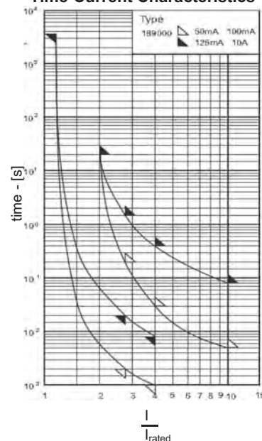
Time-Current Characteristics
