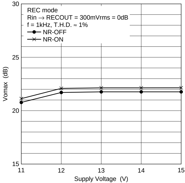
Signal Handling (1)
