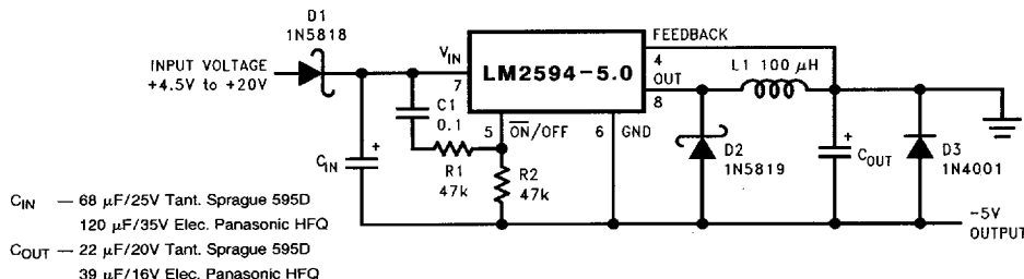
FIGURE 25. Inverting -5V Regulator with Delayed Startup
