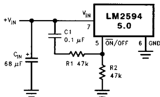
FIGURE 21. Delayed Startup
