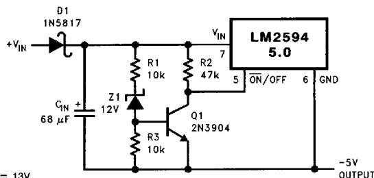
FIGURE 24. Undervoltage Lockout with Hysteresis for Inverting Regulator
