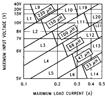
FIGURE 5. LM2594-3.3
