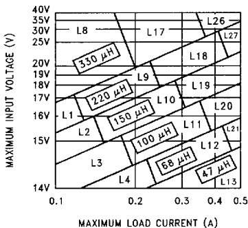
FIGURE 7. LM2594-12
