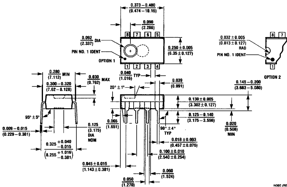
8-Lead (0.300" Wide) Molded Dual-In-Line Package, Order Number LM2594N-3.3, LM2594N-5.0, LM2594N-12 or LM2594N-ADJ NS Package Number N08E
