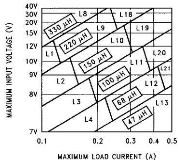
FIGURE 6. LM2594-5.0
