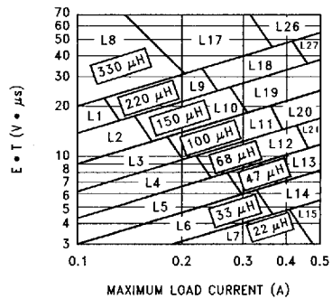
FIGURE 8. LM2594-ADJ
