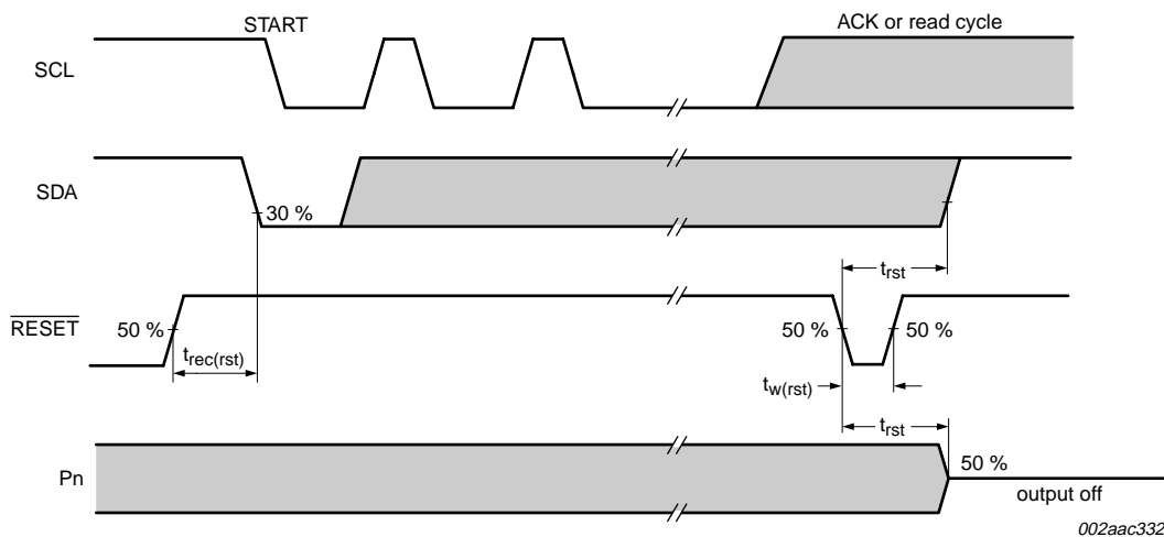
Fig 22. Reset timing
