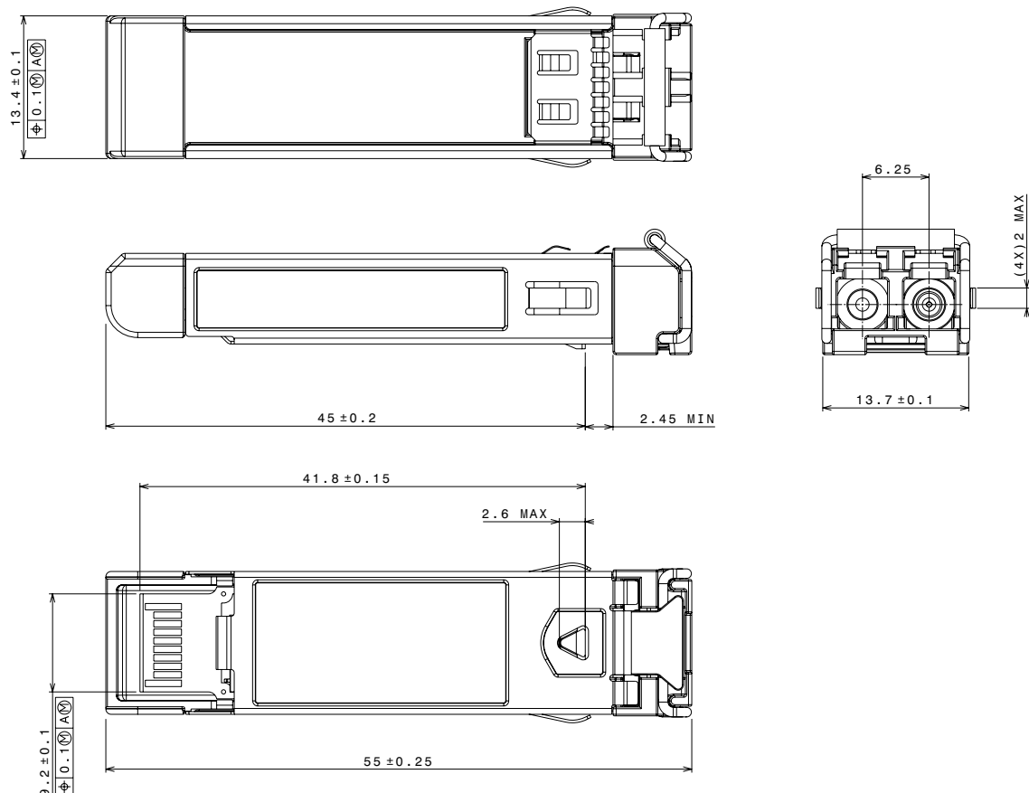
Dimensions Diagram
