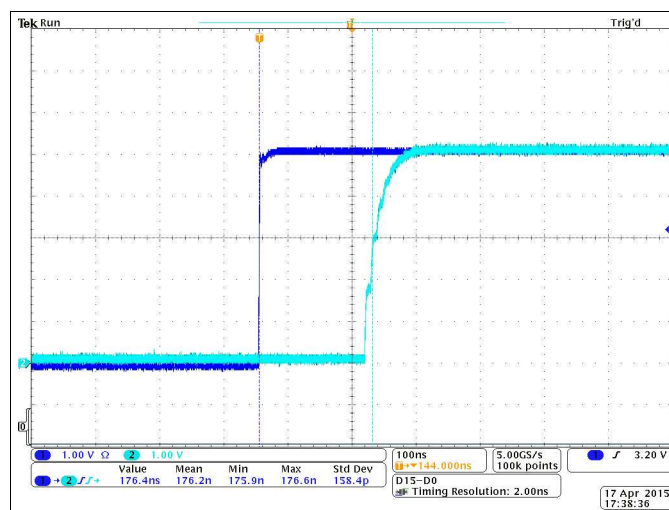
Figure 24. t_{\text{LOOP}} Delay Waveform Dominant to Recessive
