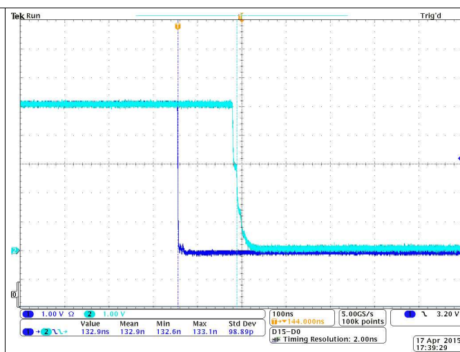
Figure 25. t_{\text{LOOP}} Delay Waveform Recessive to Dominant
