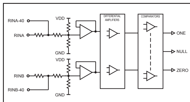
Figure 3. ARINC Receiver Input
