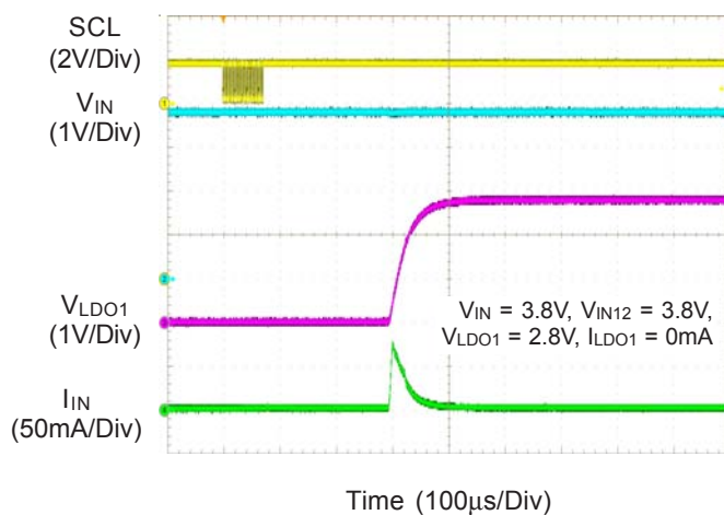
LDO1 Power On
