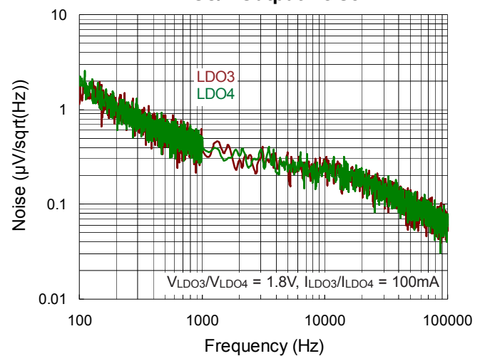
LDO3/4 Output Noise
