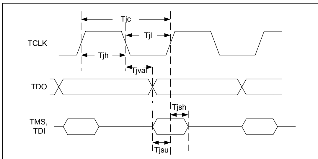
Figure 34 JTAG Timing
