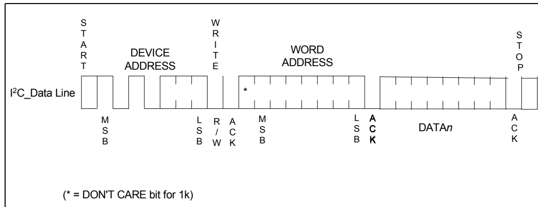
Figure 22 Byte Write
