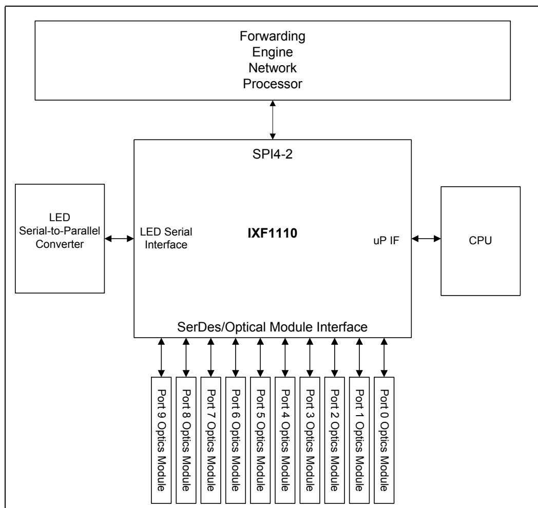
Figure 2 IXF1110 MAC System Block Diagram
