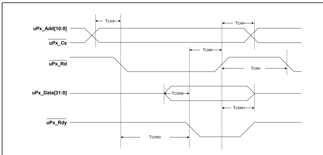
Figure 32 CPU Port Read Timing
