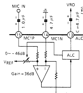
Figure 2 Microphone amp with ALC
