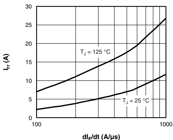
Fig. 12 - Typical I_{tr} Diode vs. dI_F/dt V_{RR} = 200\text{ V} , I_F = 50\text{ A}
