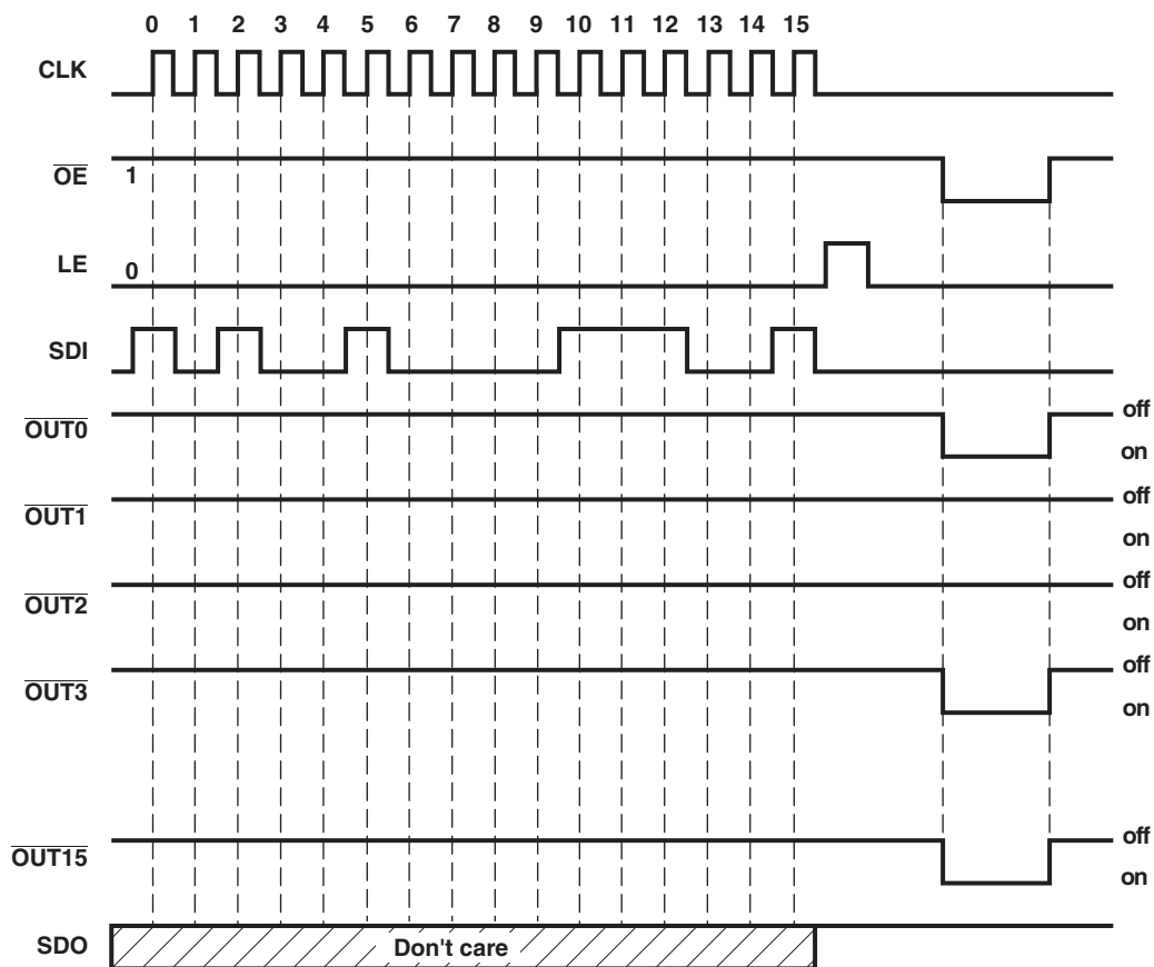
Figure 1. Timing Diagram
