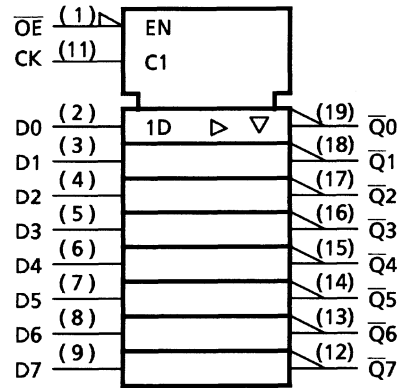
TC74HC564A
