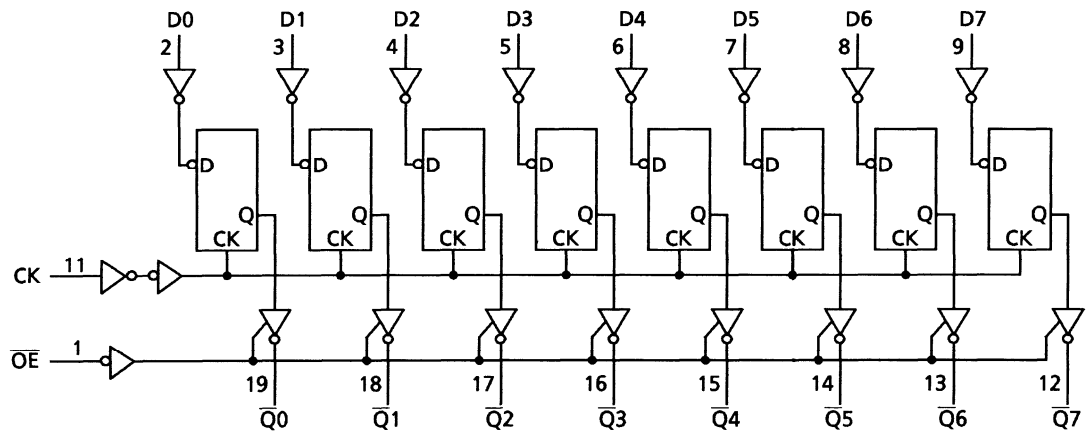
TC74HC564A
