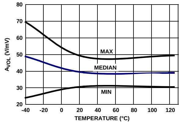
FIGURE 33. A_{VOL} vs TEMPERATURE, R_L = 1k , V_+ , V_- = \pm 2.5V , V_O = -2V TO +2V
