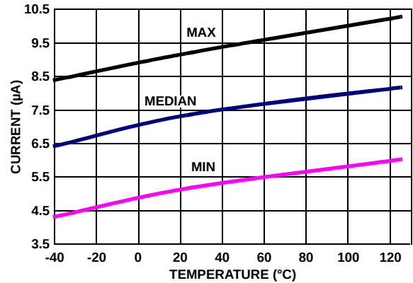
FIGURE 21. SUPPLY CURRENT DISABLED vs TEMPERATURE V_+ , V_- = \pm 2.5V
