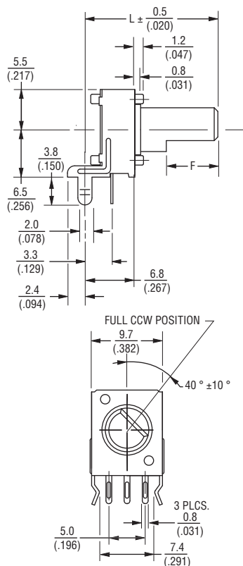
PTV09A-3 (Vertical/Side Mount, Bushingsless, 6.5 mm Height)
