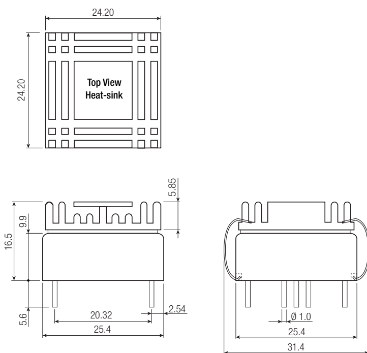
Dimension Drawing (mm) with Heat-sink
