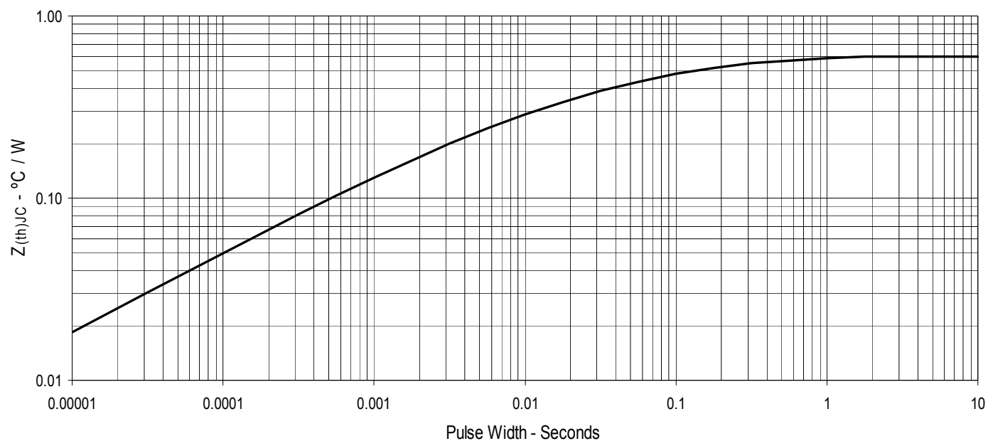
Fig. 19. Maximum Transient Thermal Impedance
