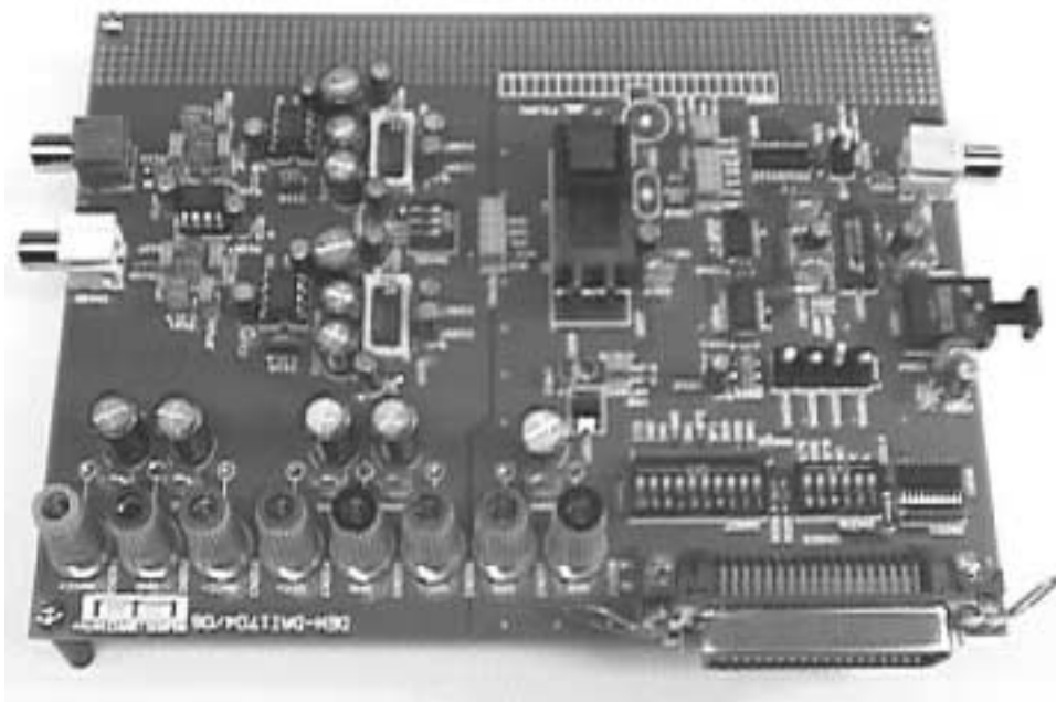
Figure 1–1. DEM-DAI1704/06 Board
