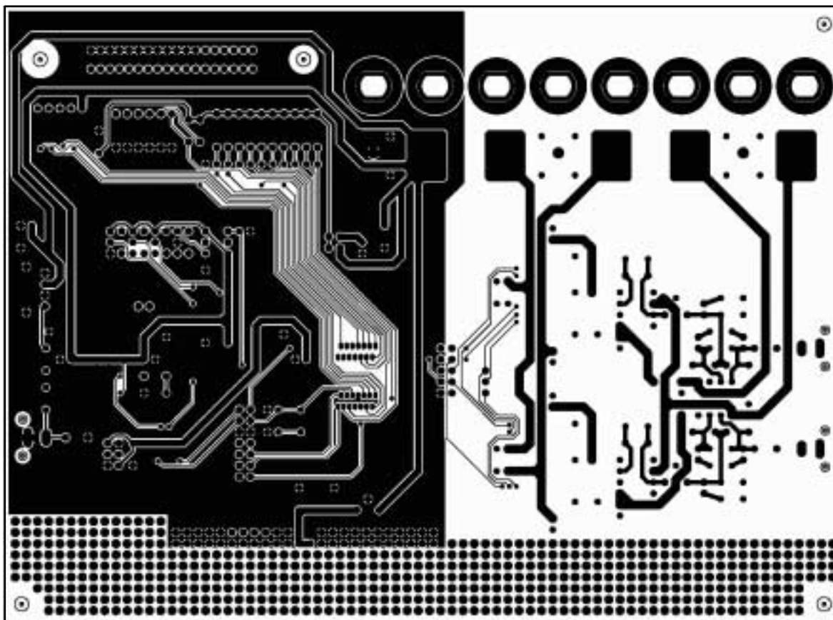
Figure 2–5. Board Layout—Bottom View
