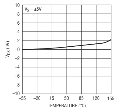
V_{\text{OS}} vs Temperature
