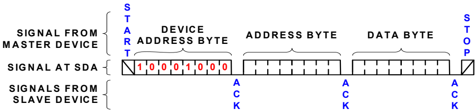
FIGURE 8. BYTE WRITE SEQUENCE
