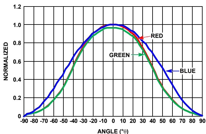
FIGURE 6. RADIATION PATTERN
