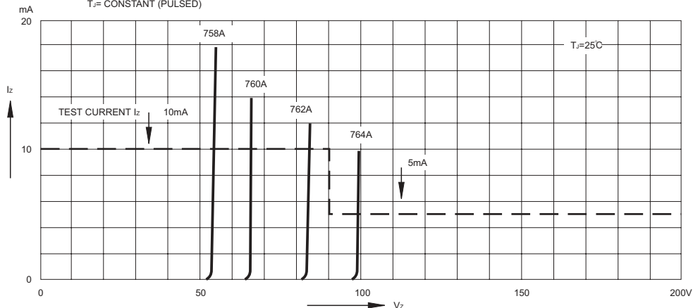
FIG.11- BREAKDOWN CHARACTERISTICS TJ = CONSTANT (PULSED)
