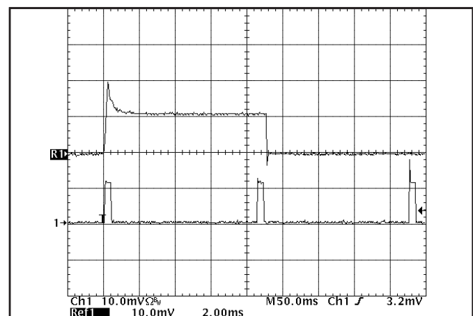
Figure 18: Load current (20A/div) as a function of time when the converter attempts to turn on into a 10 m \Omega short circuit. Top trace (2.0ms/div) is an expansion of the on-time portion of the bottom trace.
