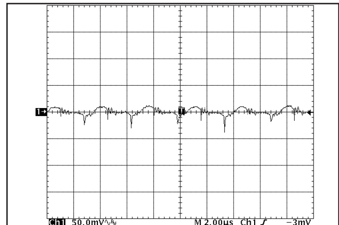
Figure 16: Output voltage ripple at nominal input voltage and rated load current (50 mV/div). Load capacitance: 1 \mu F ceramic capacitor and 10 \mu F tantalum capacitor. Bandwidth: 20 MHz. See Figure 13.
