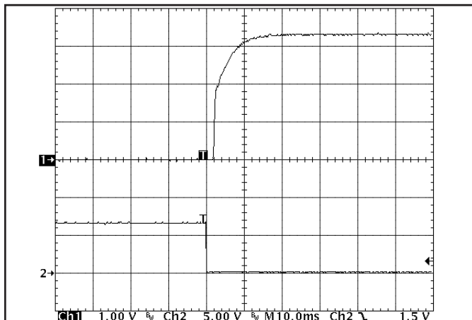
Figure 9: Turn-on transient at full load (resistive load) (10 ms/div). Ch 1: V_{out} (1V/div) Ch 2: ON/OFF input (5V/div)
