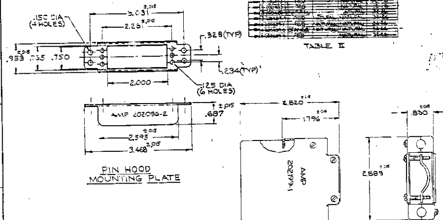
SHIELD ASSY
