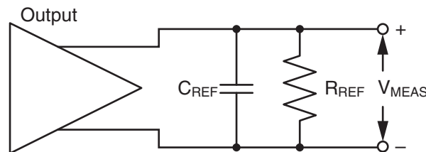
Figure 19: Differential Test Setup
