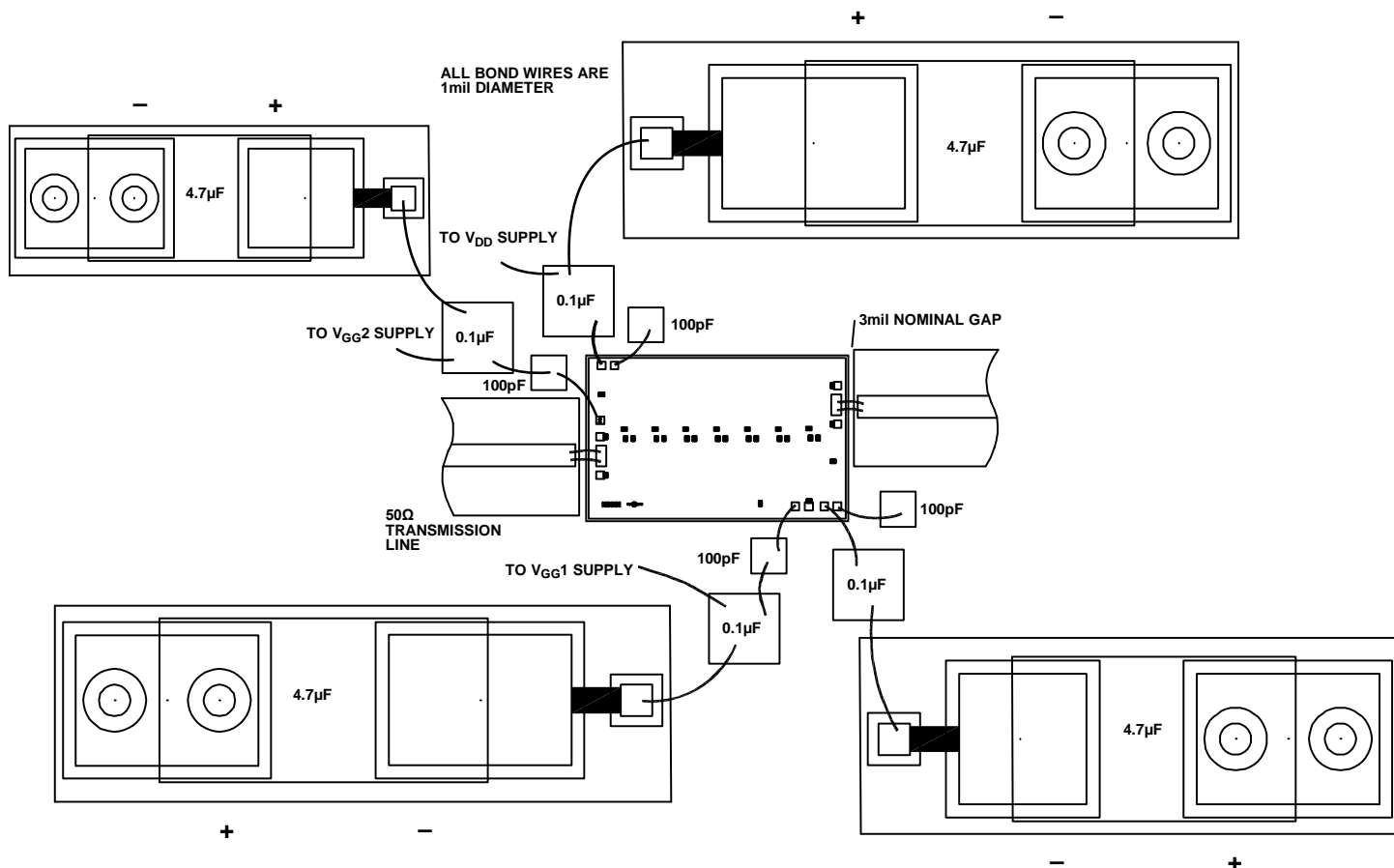
Figure 45. Assembly Diagram
