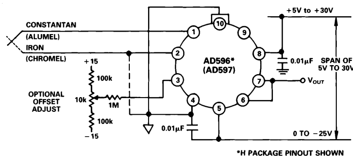
Figure 1. Temperature Proportional Output Connection
