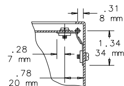
DETAIL X 87799584
