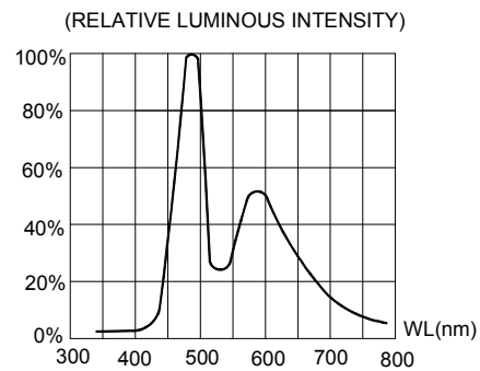
FIG.4 RELATIVE LUMINOUS INTENSITY VS. WAVELENGTH. 50% Power Angle : 120° (RELATIVE LUMINOUS INTENSITY)
