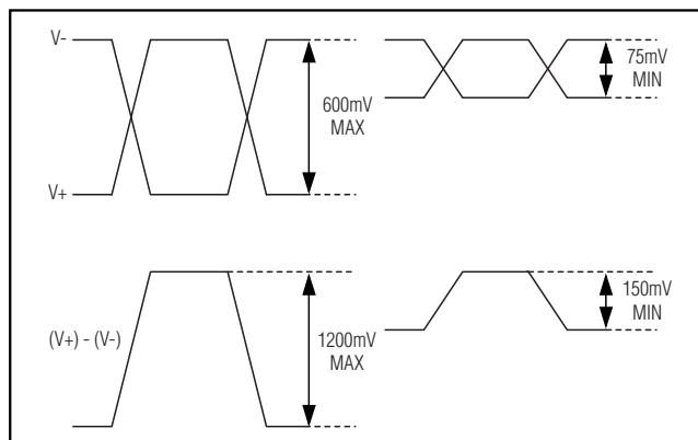
Figure 2. Definition of Differential Voltage Swing
