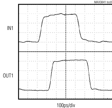
PROPAGATION DELAY
