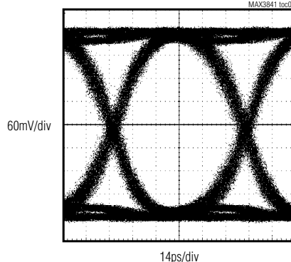
OUTPUT EYE DIAGRAM (12.5Gbps, 2^{23} - 1 PRBS)
