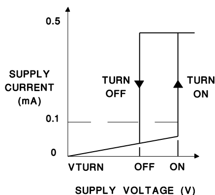
Figure 7-1. IC Supply Current at UVLO
