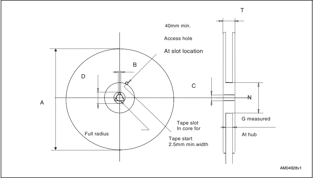
Figure 14. Reel schematic
